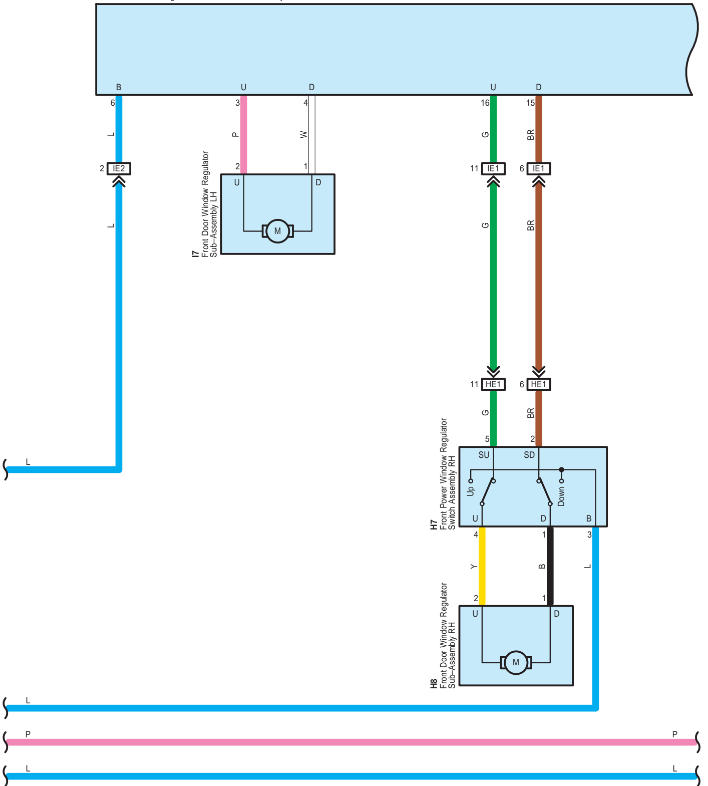
I3 Power Window Regulator Master Switch Assembly
