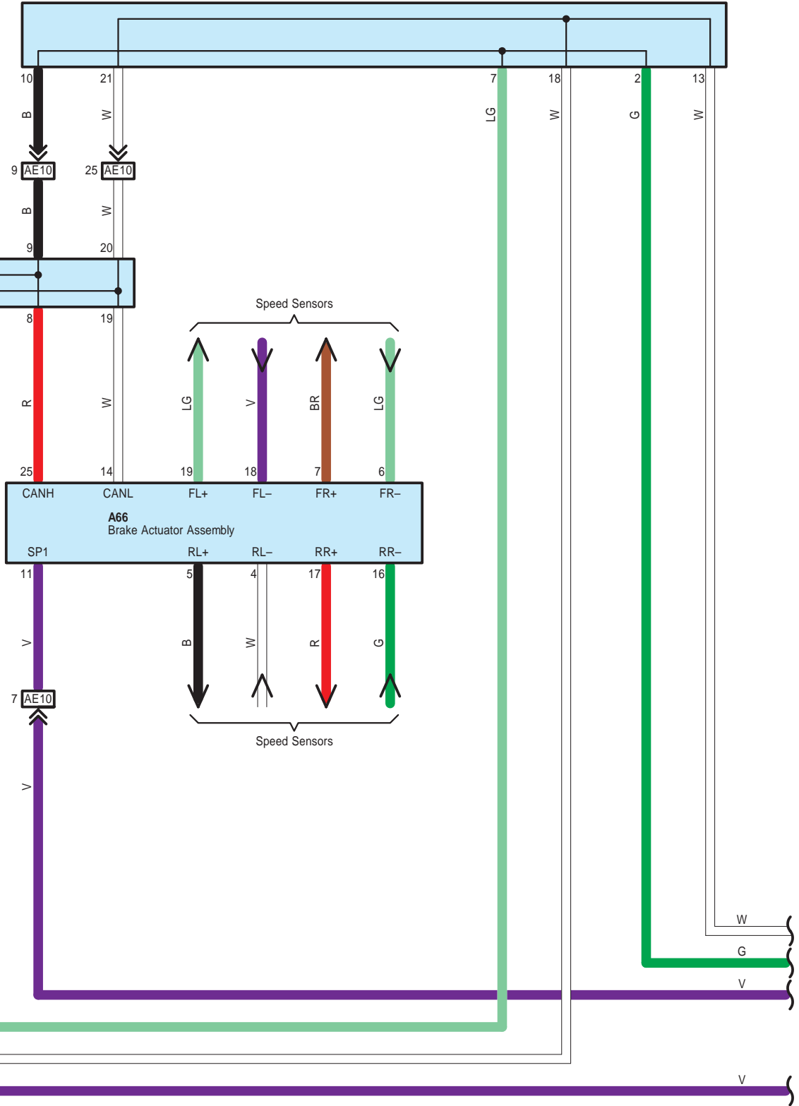
E58 Junction Connector
