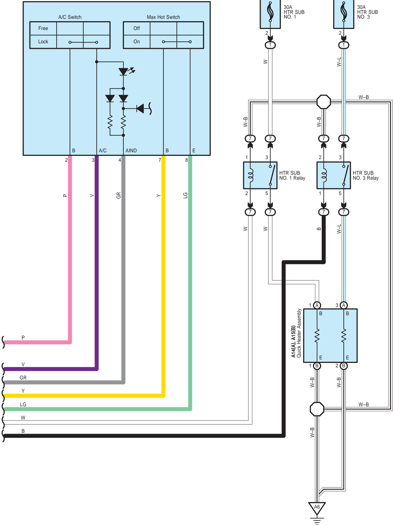
E65 No. 3 Heater Control Sub-Assembly
