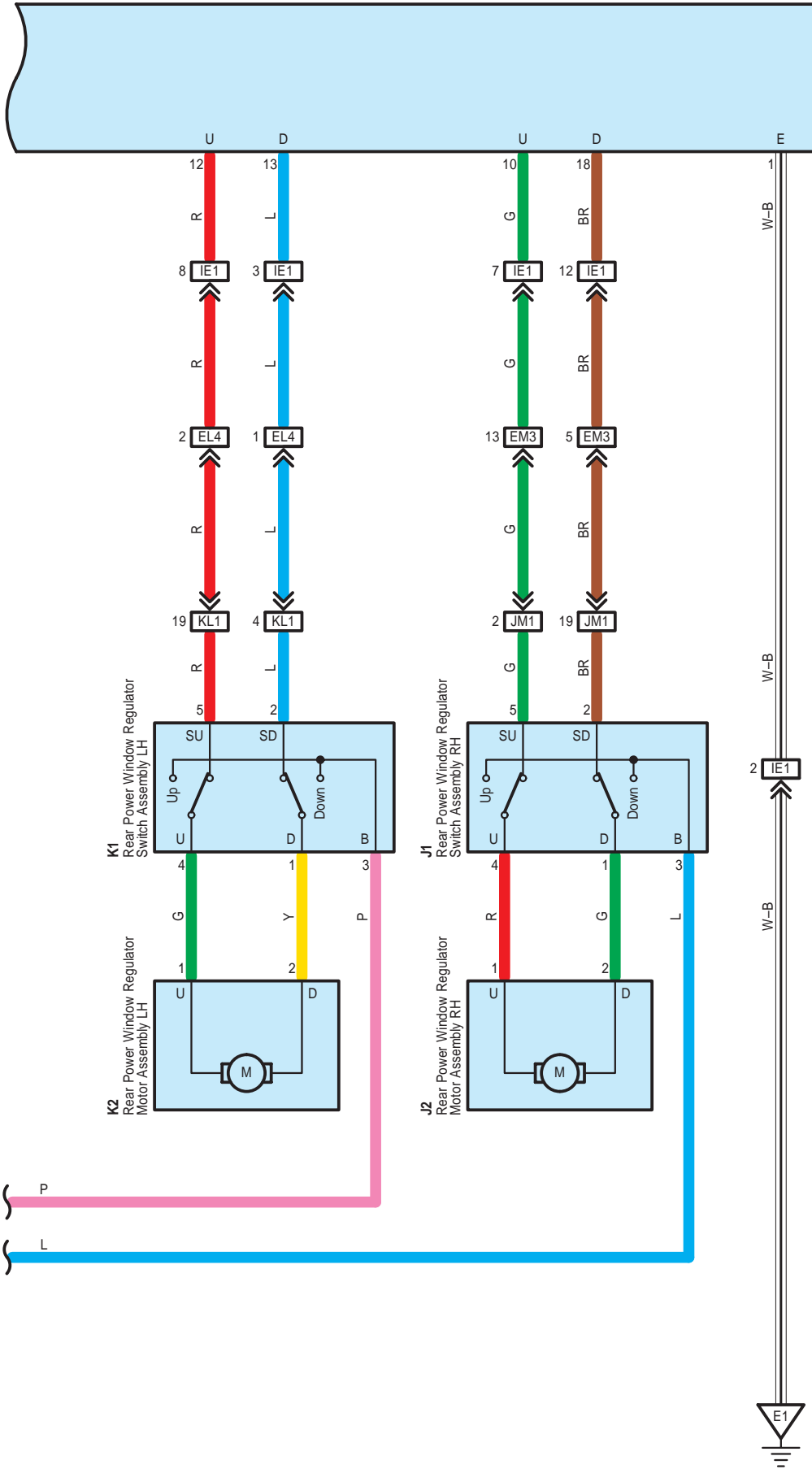
13 Power Window Regulator Master Switch Assembly
