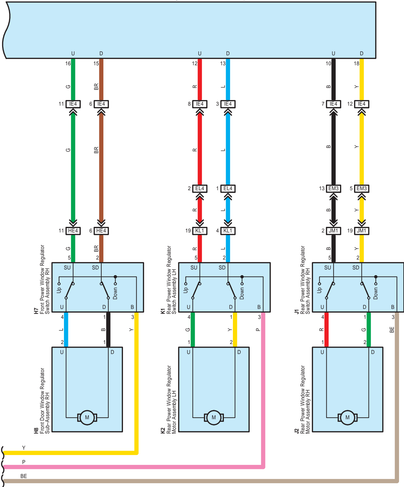
I3 Power Window Regulator Master Switch Assembly
